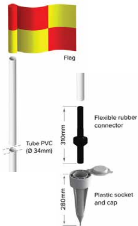
S12350-01 - BANDEIROLA / POLE W/FLAG Ø34MM
